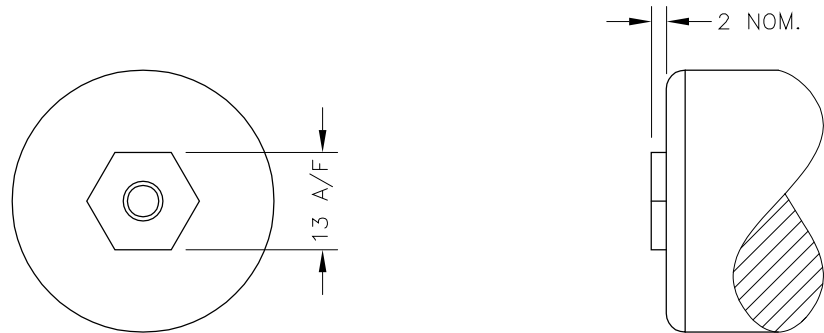
IP67 SHORT CABLE GLAND - AXIAL (CODE 'Mxx'/'MQxx')
